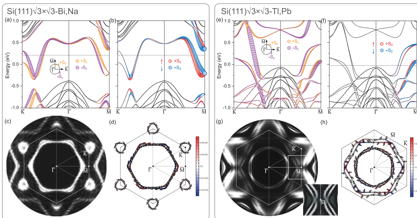
Figure 3 | Calculated band structure of the (\text{Bi, Na})/\text{Si}(111)\sqrt{3} \times \sqrt{3} (left panel) and (\text{Tl, Pb})/\text{Si}(111)\sqrt{3} \times \sqrt{3} (right panel) including spin-orbit coupling illustrating the (a, e) in-plane and (b, f) out-of-plane polarization components. (c, g) Experimental and (d, h) calculated Fermi contours. Inset in (g) shows the fine structure within the outlined area around the \bar{M} point with a greater contrast. Arrows adjacent to the calculated contours and their length denote the in-plane spin component. The out-of-plane spin component is indicated by the color with red and blue corresponding to the upward and downward directions, respectively. White colour indicates fully in-plane spin alignment. The tic values in parentheses in (d) refer to the pocket contours around the \bar{K} .
